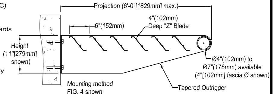
SECTION "A"
